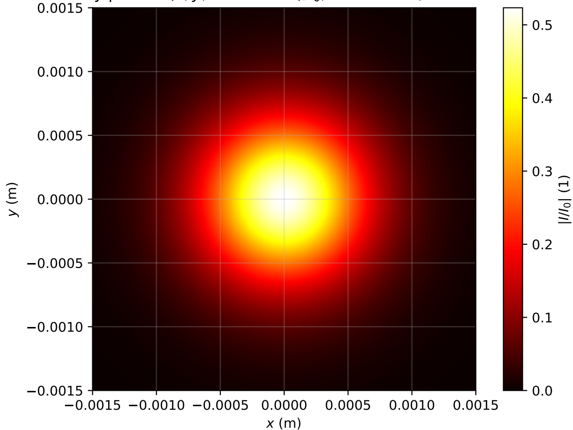
Intensity profile I(x, y, z = 3.742m)/I_0 , \text{Pin}=0.6\text{Pcr} , artificial time
